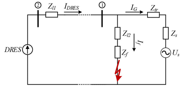
Fig. 9 Equivalent circuit for voltage versus PF calculation
