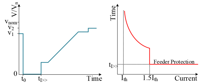
Fig. 10 Relation of FRT curve with protection curve
