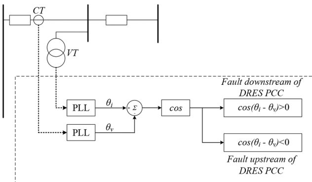
Fig. 8 Fault location detection
