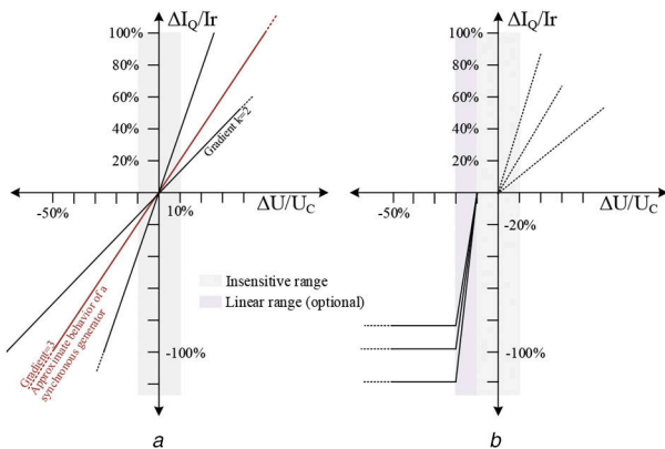
Fig. 18 Reactive power injection during voltage sags according to (a) Standard 50549:2019, (b) Proposed method
