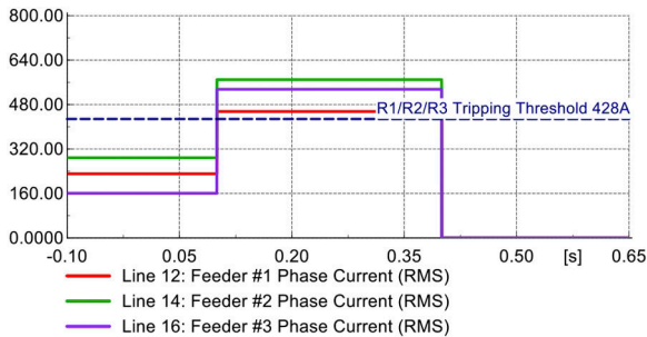
Fig. 16 Maximum fault contribution by CI-DRES. Fault currents in each feeder
