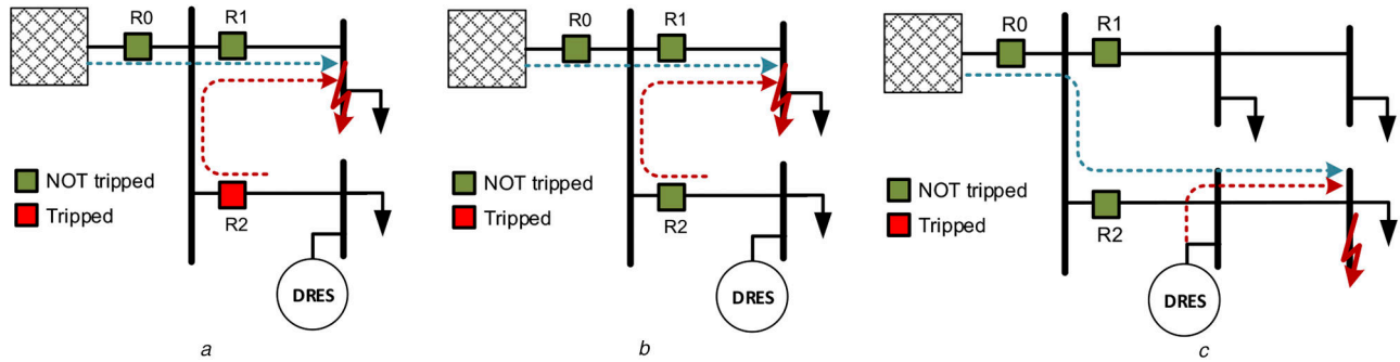
Fig. 1 Protection problems (a) Sympathetic tripping, (b) Blinding of back up protection, (c) Blinding of feeder protection
