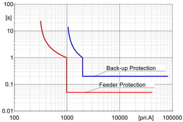
Fig. 2 Protection curves for feeder and back-up protection
