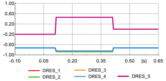
Fig. 14 Value of \cos(\theta_i - \theta_v) for fault position detection
