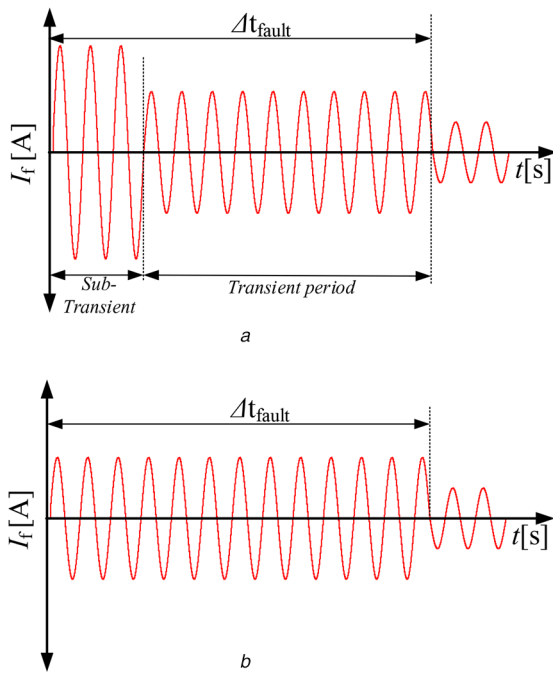
Fig. 4 CI-DRES fault current (a) With sub-transient and transient part, (b) With transient part only
