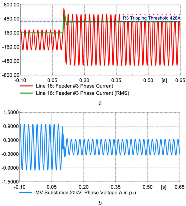
Fig. 11 CI-DRES injecting nominal current (a) Fault current in feeder 3, (b) Voltage of main Bus_1
