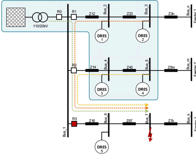
Fig. 3 Protection philosophy for weak distribution grids with a high share of CI-DRES
