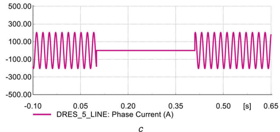
Fig. 13 Fault current injected by each CI-DRES (a) In feeder 1, (b) In feeder 2, (c) In feeder 3
