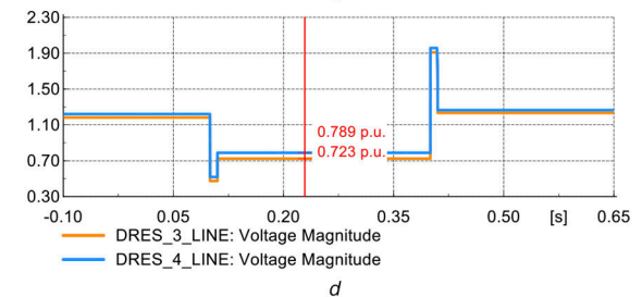
Fig. 15 Proposed CI-DRES reaction ( PF = 0.1 ) (a) Fault current in feeder 3, (b) Voltage of main Bus_1, (c) Voltage of DRES 1 and 2 PCC, (d) Voltage of DRES 3 and 4 PCC
