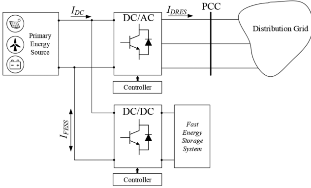
Fig. 5 CI-DRES converter topology
