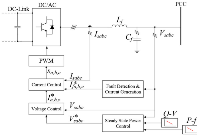
Fig. 6 CI-DRES converter control
