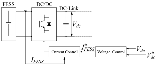
Fig. 7 FESS control
