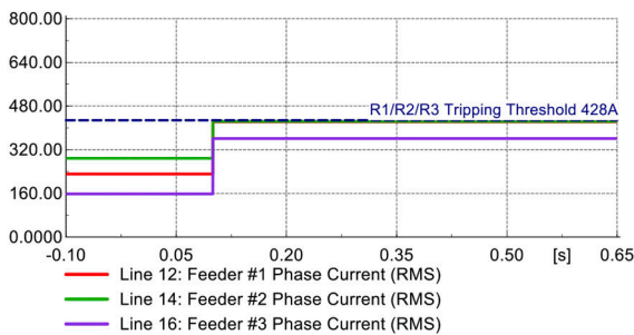
Fig. 17 CI-DRES fault contribution irrespective of the fault location. Fault currents in each feeder
